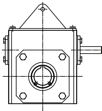
Torque Arm 375 - 600
